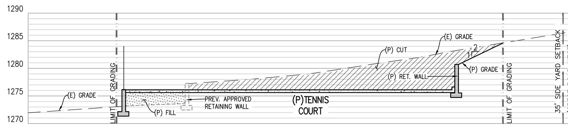
SECTION B- TENNIS COURT SCALE: 1" = 10'
