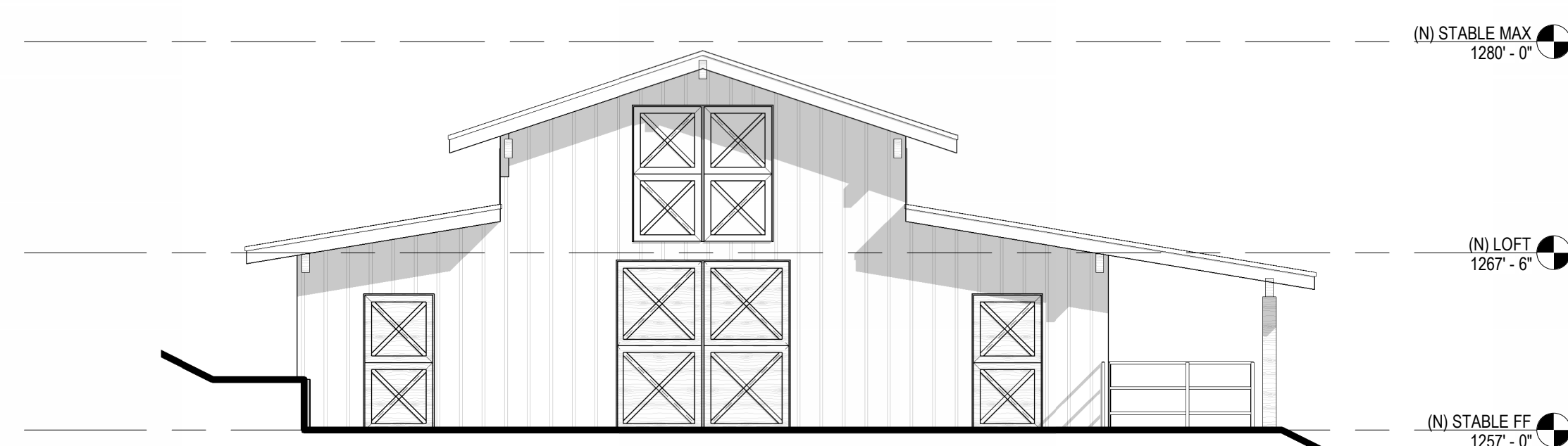
STABLE S REAR \frac{1}{8}" = 1'-0" 03
