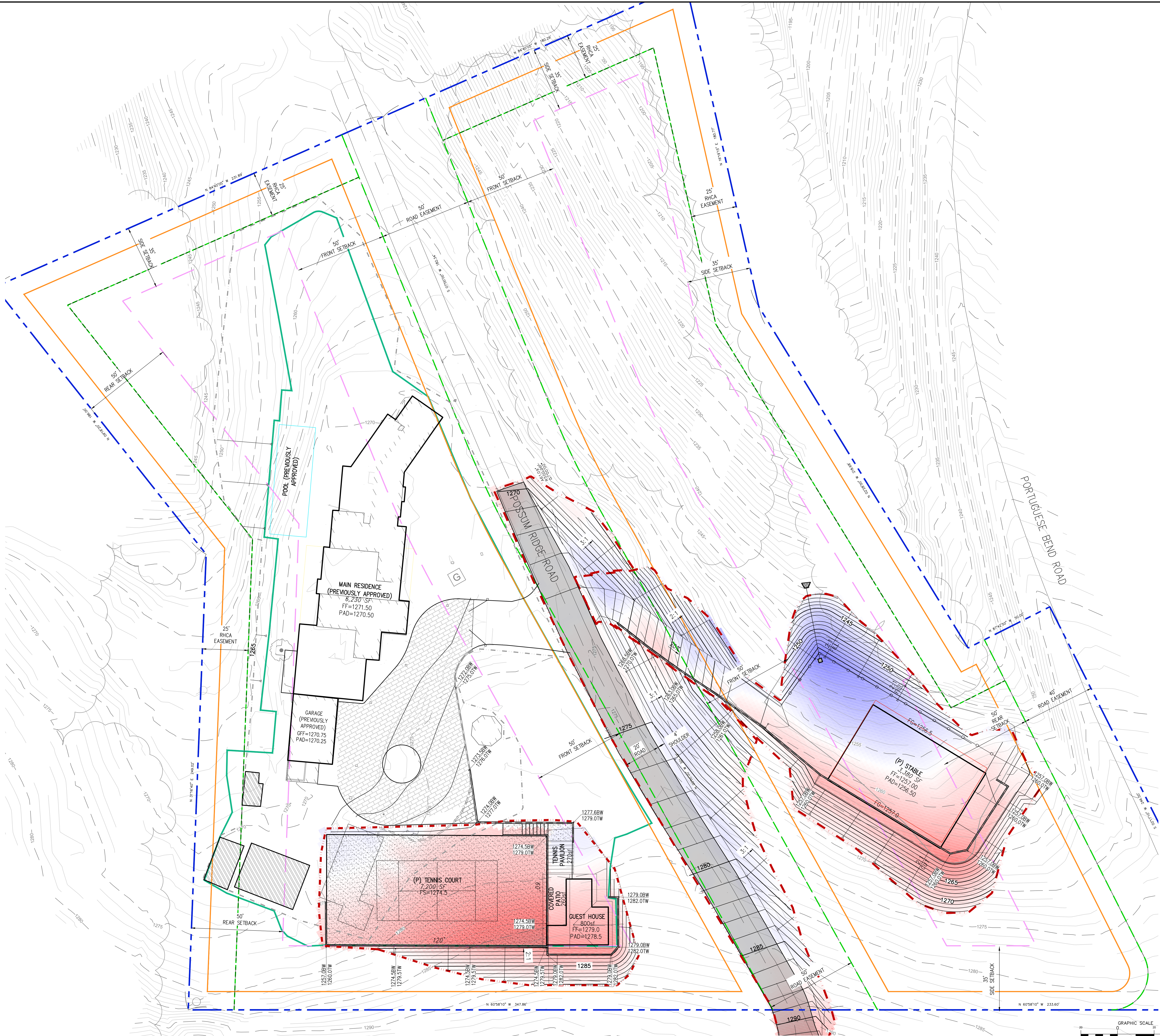
CUT - FILL AND COLOR MAP SCALE: 1" = 20'
