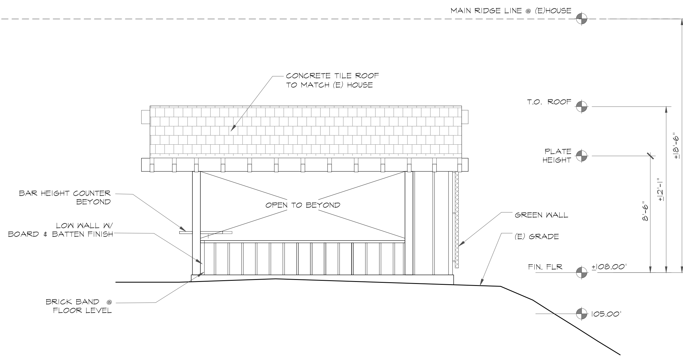
3 WEST ELEVATION Scale: 1/4" = 1'-0"
