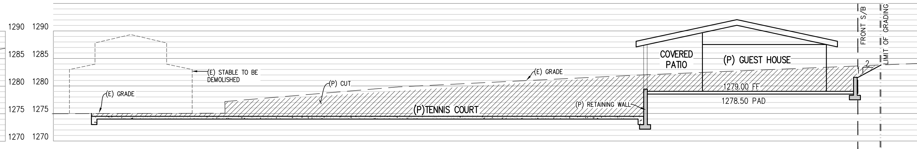
SECTION A- TENNIS COURT SCALE: 1" = 10'
