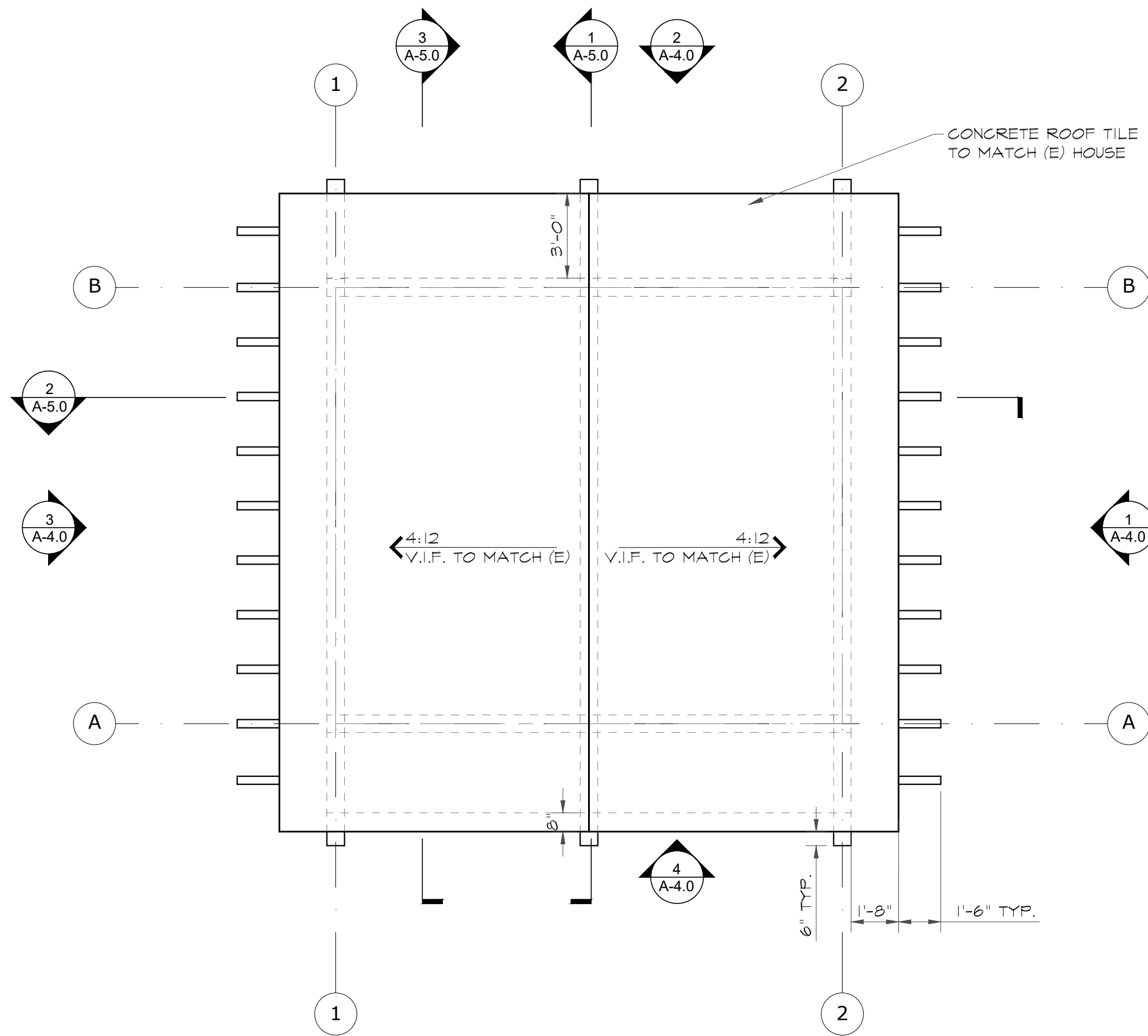
2 Proposed Roof Plan
