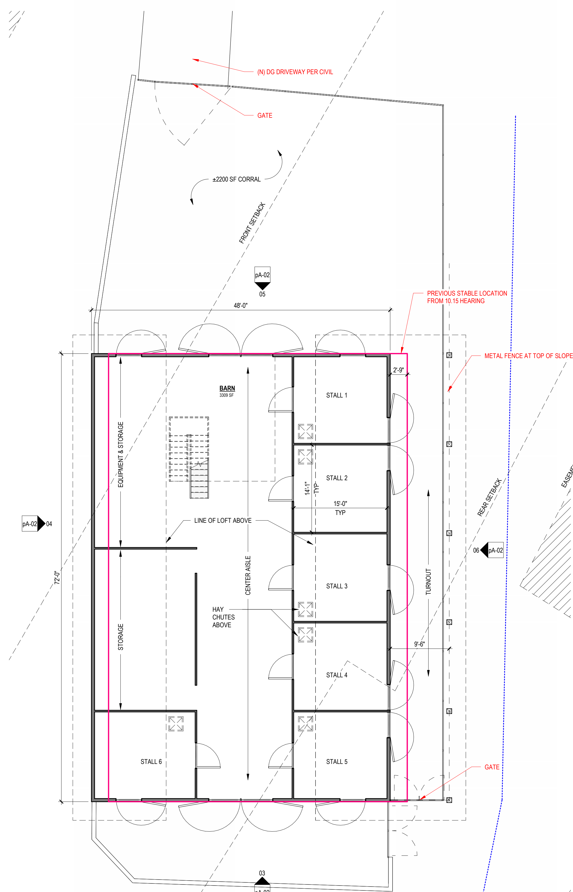
STABLE 01 1/8" = 1'-0"
