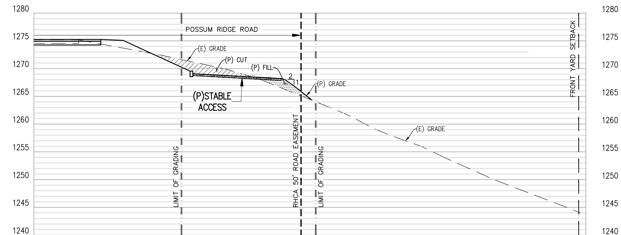
SECTION D - STABLE SCALE: 1" = 10'
