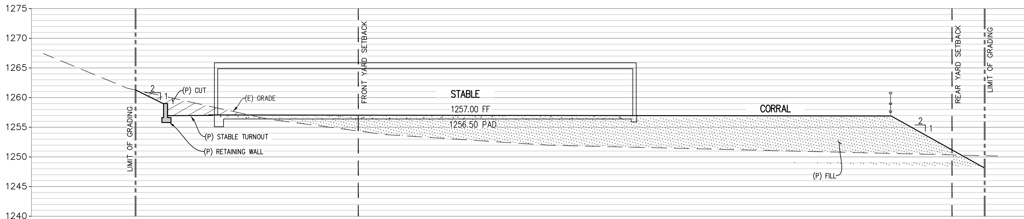
SECTION D - STABLE SCALE: 1" = 10'
