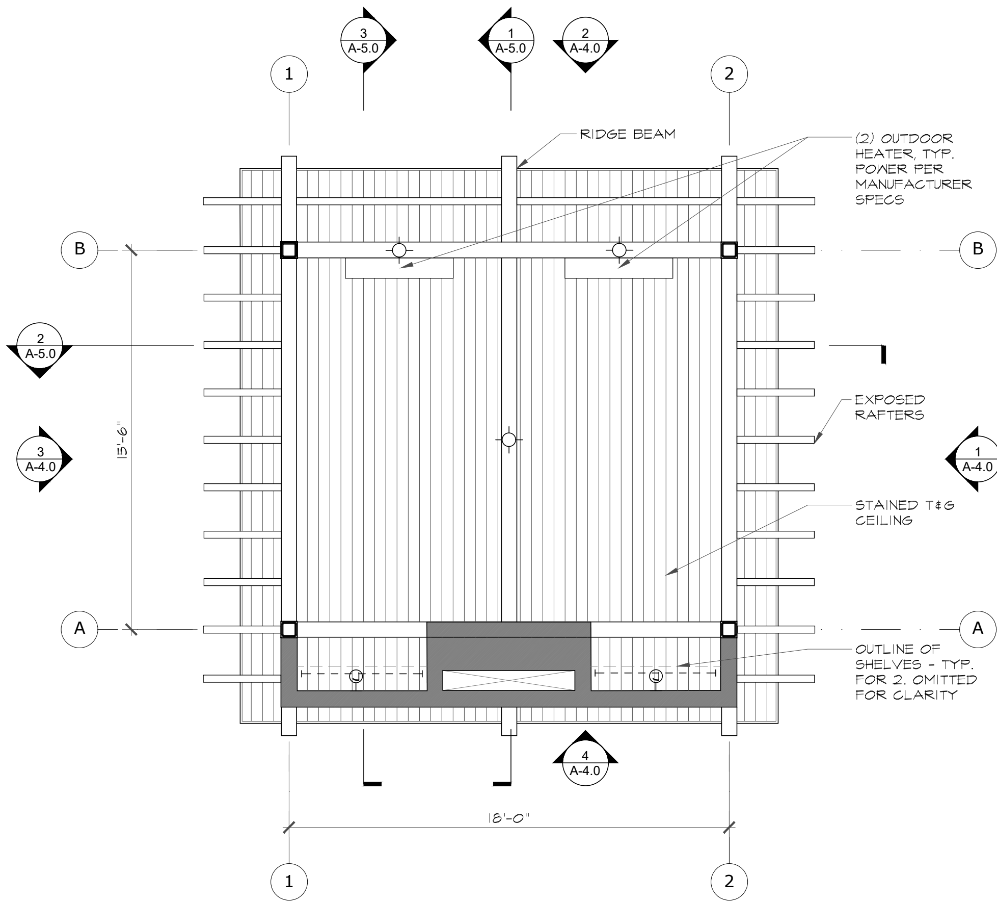
4 Proposed Reflected Ceiling Plan
