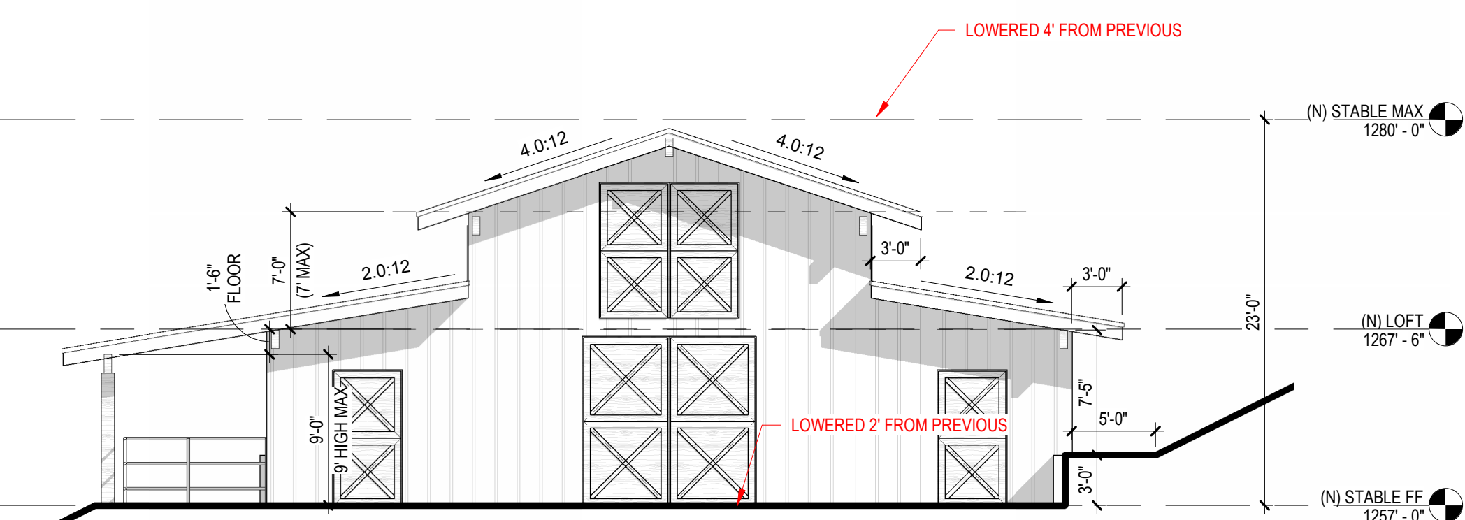
STABLE N FRONT 05 1/8" = 1'-0"
