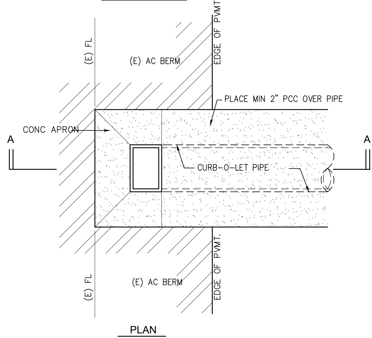
DRAIN OUTFALL THROUGH AC BERM SCALE: NTS
