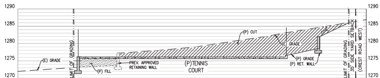
SECTION B- TENNIS COURT SCALE: 1" = 10'
