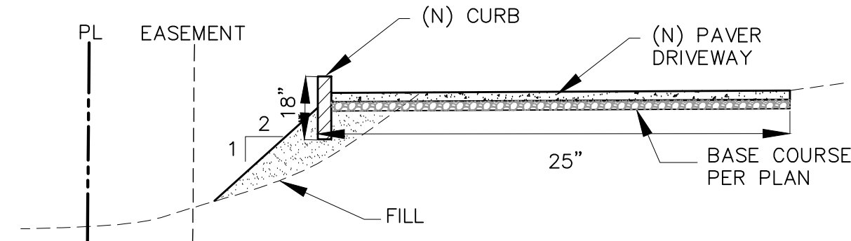
TYPICAL DRIVEWAY SECTION NTS
