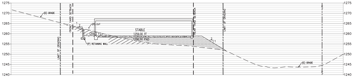
SECTION C - STABLE SCALE: 1" = 10'
