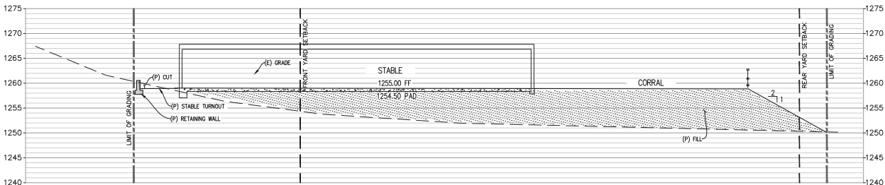
SECTION D - STABLE SCALE: 1" = 10'
