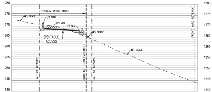
SECTION D - STABLE SCALE: 1" = 10'
